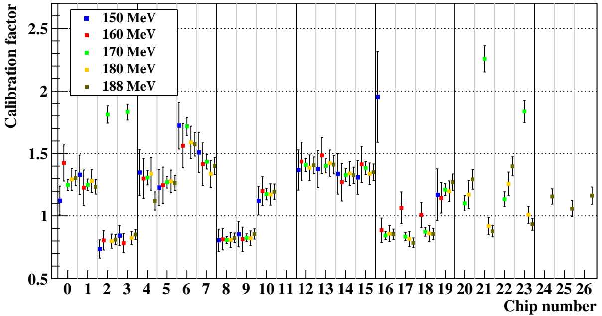
Figure 3.7: Chip sensitivity calibration factors f(\text{Chip}) , applied for obtaining a relatively uniform cluster size distribution in the different layers. For stability-checking purposes, a set of calibration factors has been made for all datasets at different energies. It is found that the calibration factors have a higher variation in the Bragg peak area for each energy, since it is harder to accurately model the energy deposition when the energy deposition is high.
