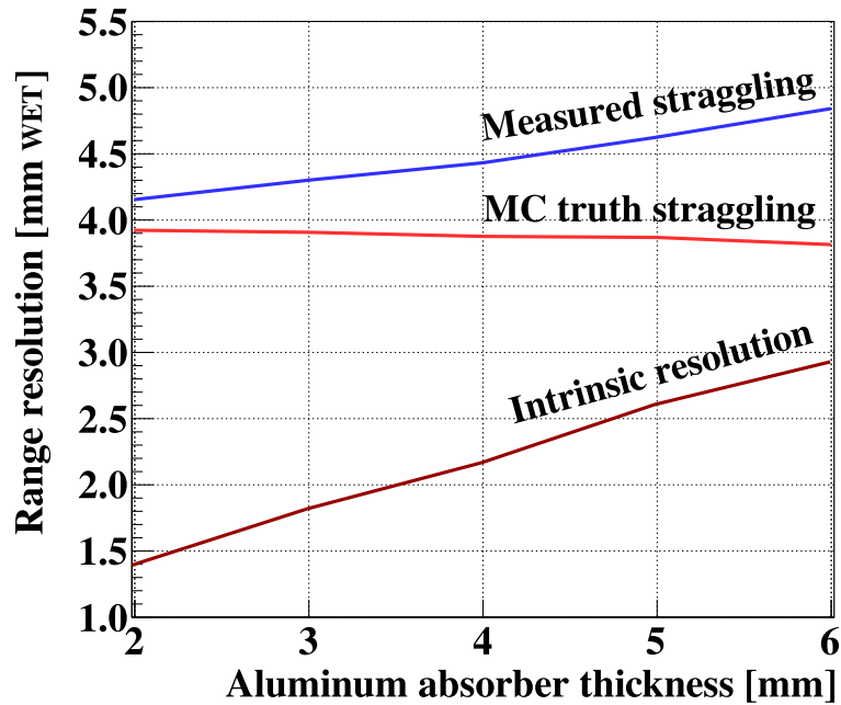
Figure 5.12: The range uncertainties for the proposed designs. Shown in the figure is the total uncertainty (measured as the mean value of \langle\sigma_R\rangle in Fig. 5.11), the range straggling from the MC truth as well as the added uncertainty which is the quadratic difference between the two. See Table 5.2 for the number of required layers for the shown designs.
