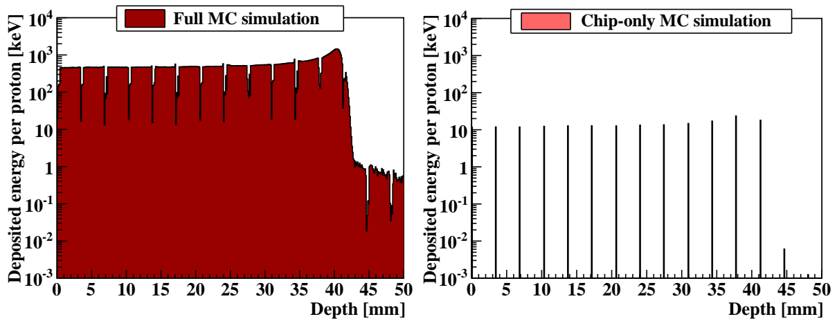
Figure 4.2: Total energy deposition in full simulations (i.e., primaries and secondaries are scored in all volumes) and chip-only simulations (i.e., only the epitaxial layers of the sensor chips are scored).
