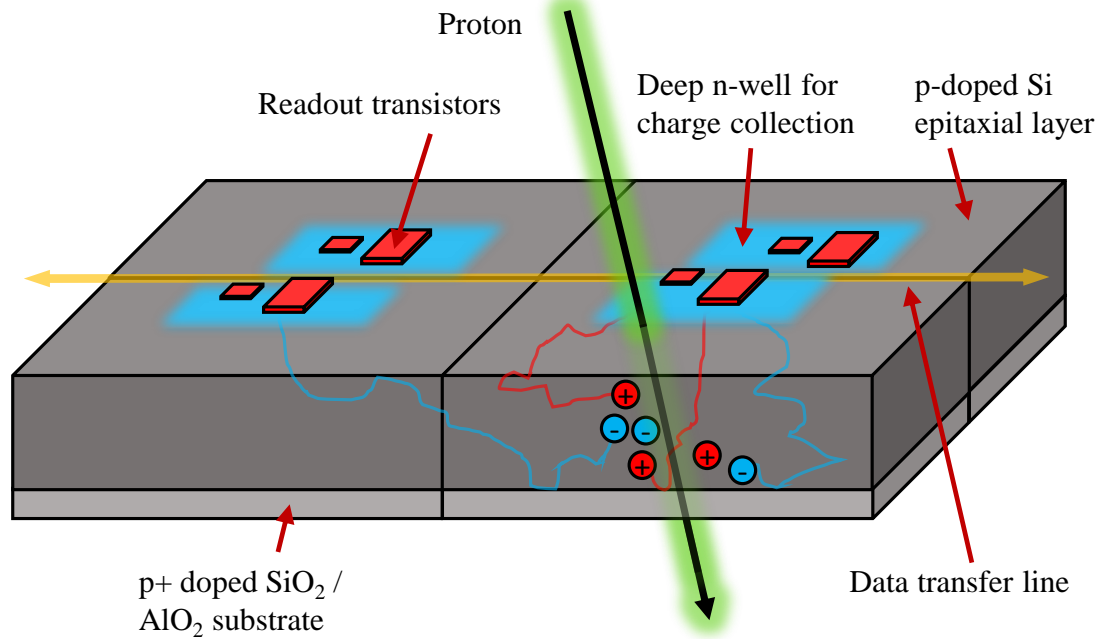
Figure 3.1: Schematics of a Monolithic Active Pixel Sensor (figure by H. E. S. Pettersen, 2017). Electron-hole pairs are liberated from the traversing charged particle in the epitaxial p-doped silicon layer. The charge carriers diffuse to the deep n-wells in the closest neighboring pixels, where they are collected. The collected charge in the deep n-well is read out through transistors, and, depending on the design, the signal is digitized before being transmitted through the data lines.
