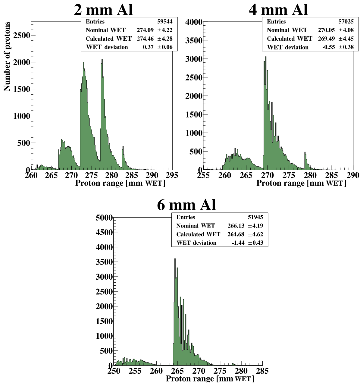
Figure 5.6: Distribution of individual estimated ranges. From this distribution the residual range \langle R \rangle and range straggling \langle \sigma_R \rangle of a proton beam is calculated, shown in the text box as “ \langle R \rangle \pm \langle \sigma_R \rangle ”. The characteristic pattern of the distribution, with regular sudden rises can be seen in the figure. Each rise in the distribution is in coincidence with the beam reaching a new sensor layer. MC data taken with a 250 MeV monoenergetic proton beam degraded using a 10 cm water phantom.
