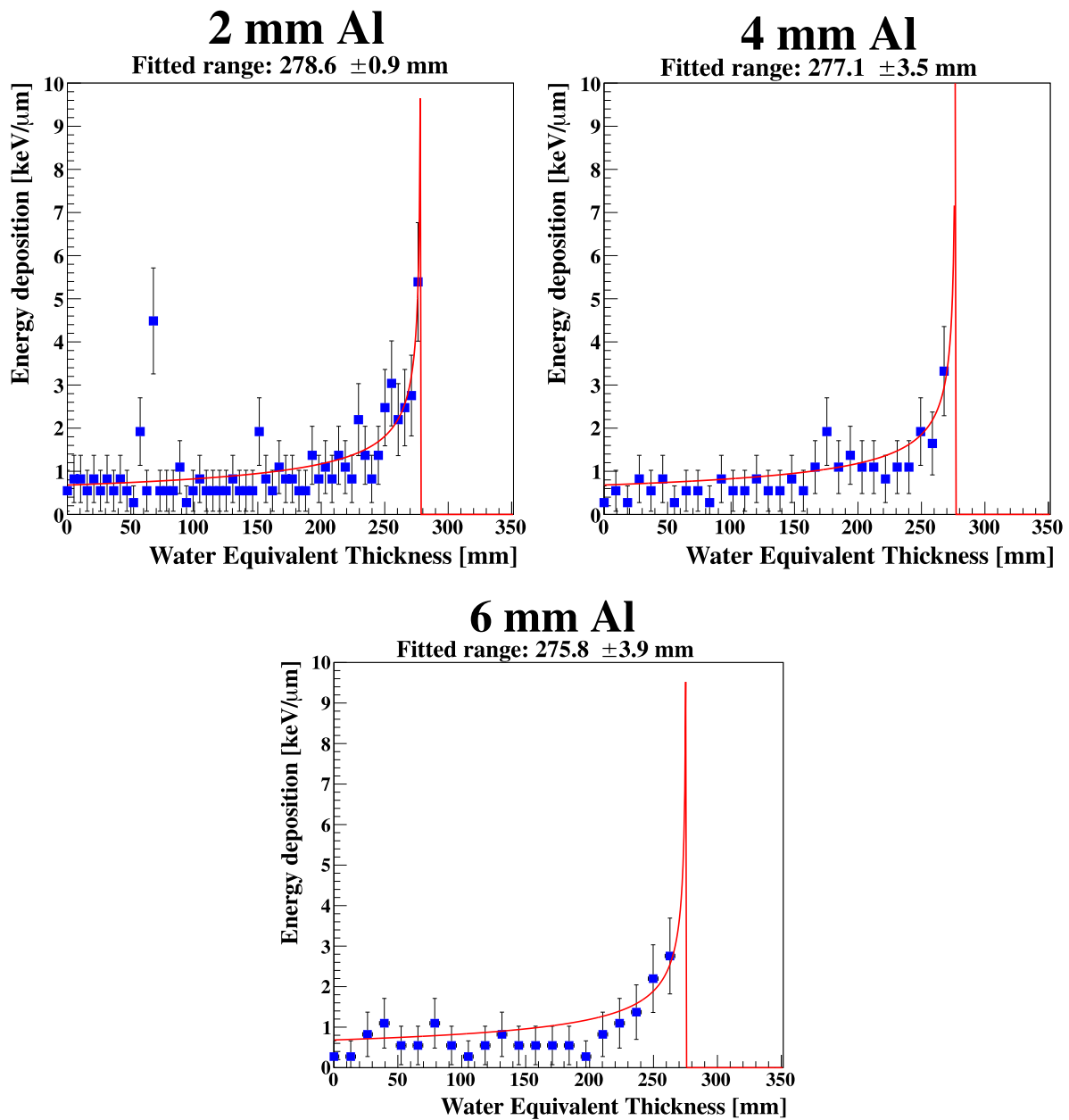
Figure 5.5: Individual 250 MeV proton tracks in three different geometries, degraded with 10 cm water phantom, overlaid with a Bragg curve fit. The displayed “ \pm ” accuracy is the output from the least-square method applied on an individual proton, and it is not representative for a proton beam of that energy. MC data taken with a 250 MeV beam degraded using a 10 cm water phantom.
