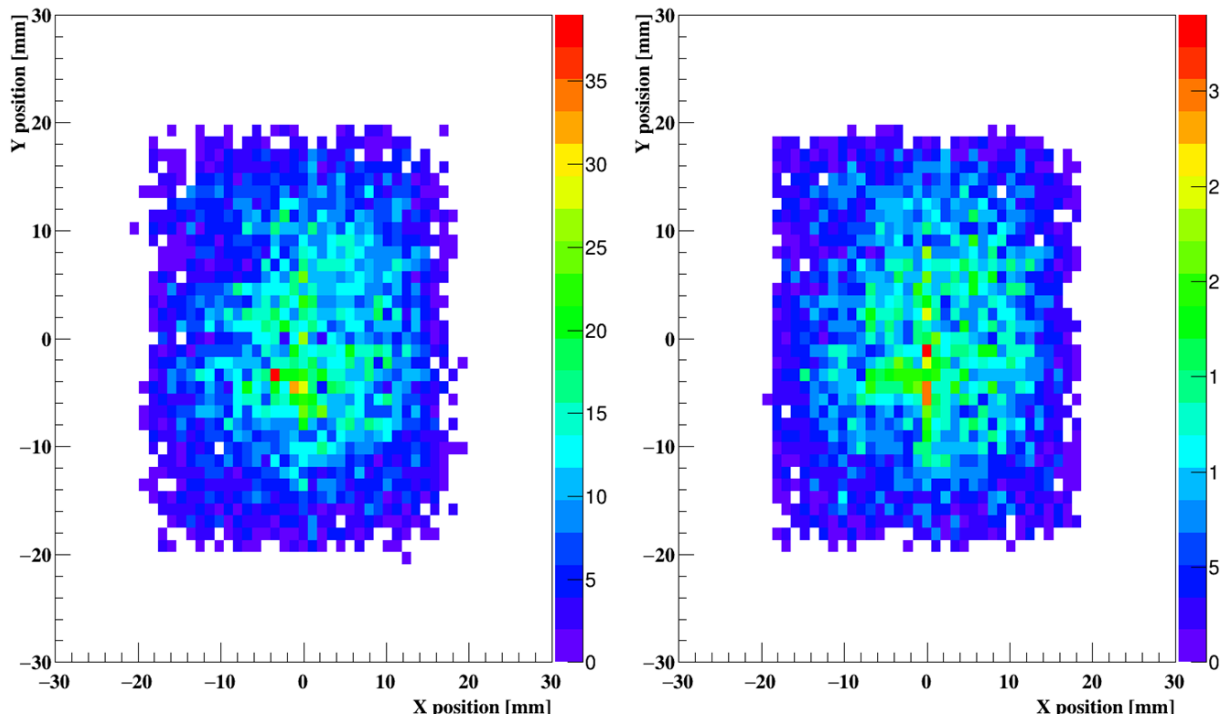
Figure 3.4: Left: Lateral position of incoming protons at the front face of the detector. Right: Lateral position of protons at their stopping position inside the detector. Both figures are constructed with experimental data at all the available proton beam energies.
