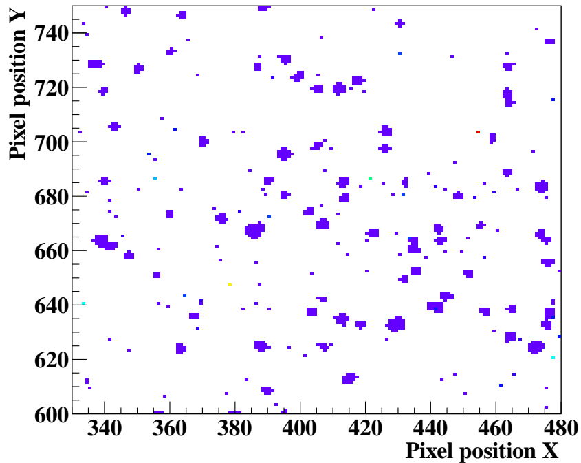
Figure 4.6: A portion of the (1280×1280) pixel hit map from the first layer in the 170 MeV beam data. Each traversing proton activate a large pixel cluster. Note features such as hot (always-activated) pixels due to their high values (in red, green and yellow), summed over many data frames, and noise, identified as single-pixel hits.
