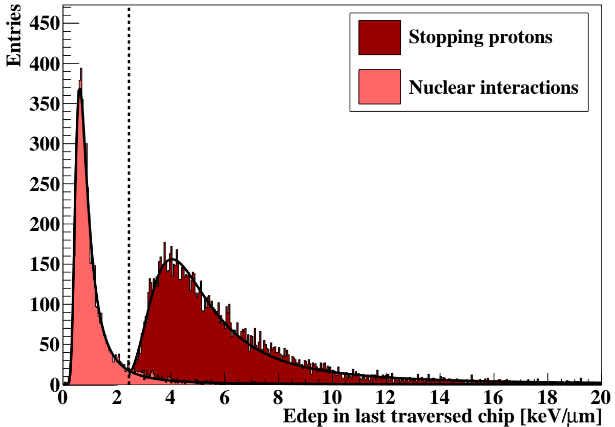
Figure 4.16: Energy loss distributions of protons stopping due to ionization energy loss and nuclear interactions, each fitted with a Landau curve. The dotted line shows the E_{dep} where the contributions from the two processes are equal, and it is used for discrimination between the two.
