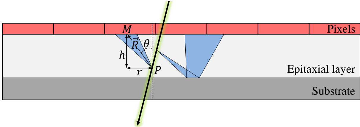
Figure 4.10: Schematics of a the proton's path through a MIMOSA23 chip (not to scale). Electron-hole-pair ionization events from the proton's path are shown as shaded conical areas.
