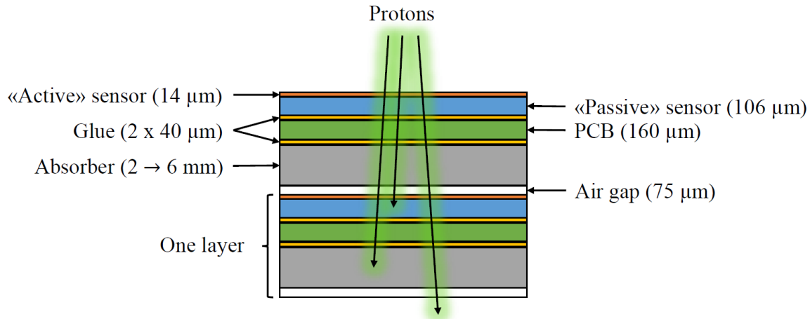
Figure 5.2: Design to be optimized: Different thicknesses (2–6 mm) for the energy absorbers are considered, and evaluated through the MC simulations. Only the “active” sensor volumes are scored in the MC simulations.
