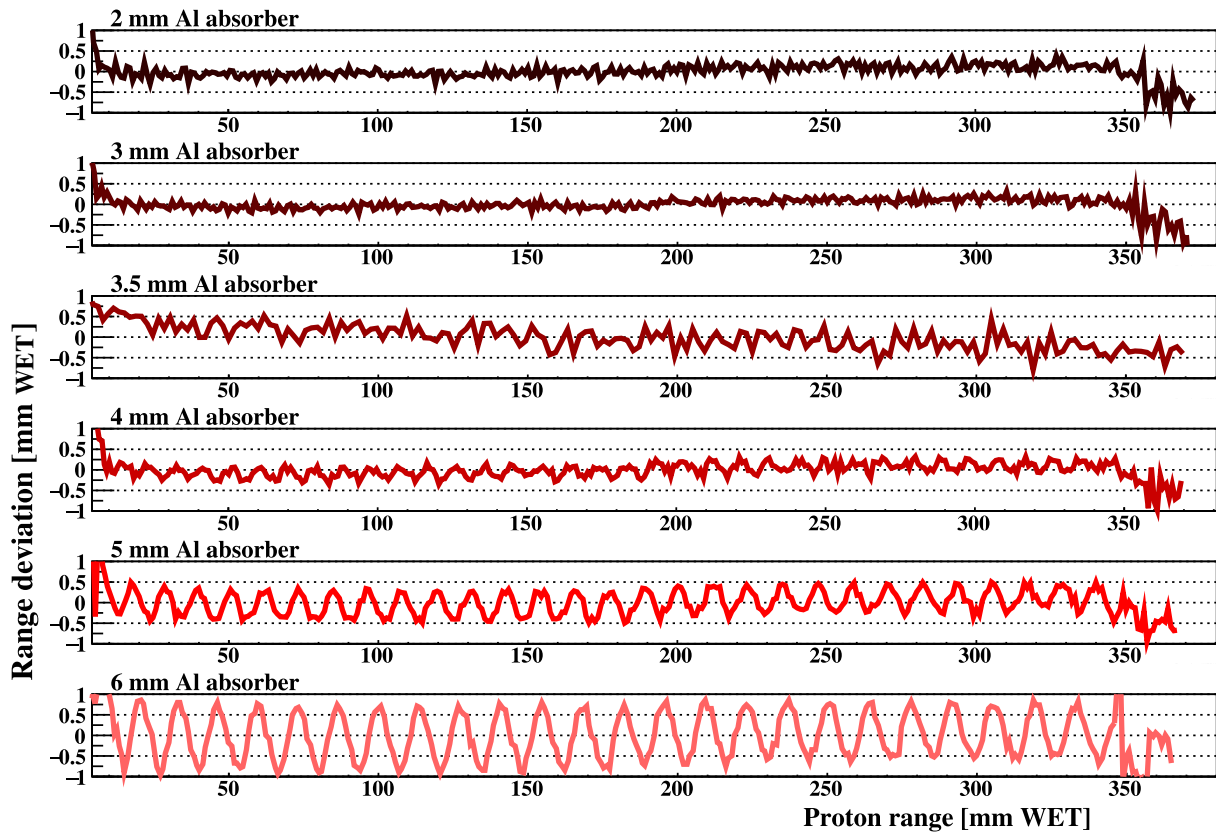
Figure 5.9: Range determination accuracy shown as the deviation between the “MC truth” range, and the reconstructed range \langle \hat{R} \rangle . For visualization purposes, a calibration constant has been added to all ranges within a given geometry: this constant is below 1 mm (below 2 mm for the 5 and 6 mm thicknesses).
