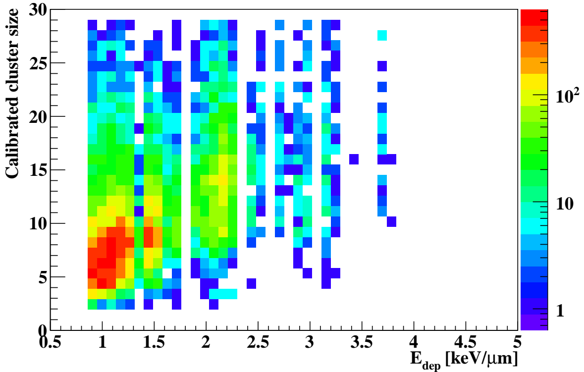
Figure 4.9: Correlation between E_{dep} and cluster sizes. The cluster sizes are calibrated using the chip sensitivity calibration factors, and the E_{dep} is calculated using energy-loss tables together with information about the sensor layer depth relative to the nominal range.
