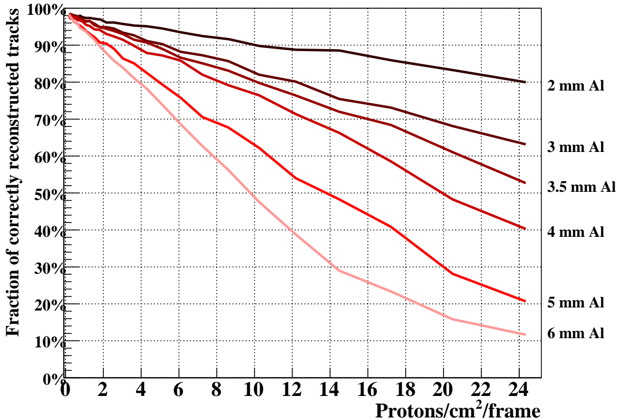
Figure 5.7: The tracking efficiency for different geometries. Each proton track must be fully reconstructed, and the start- and endpoint must originate from the same incoming proton.
