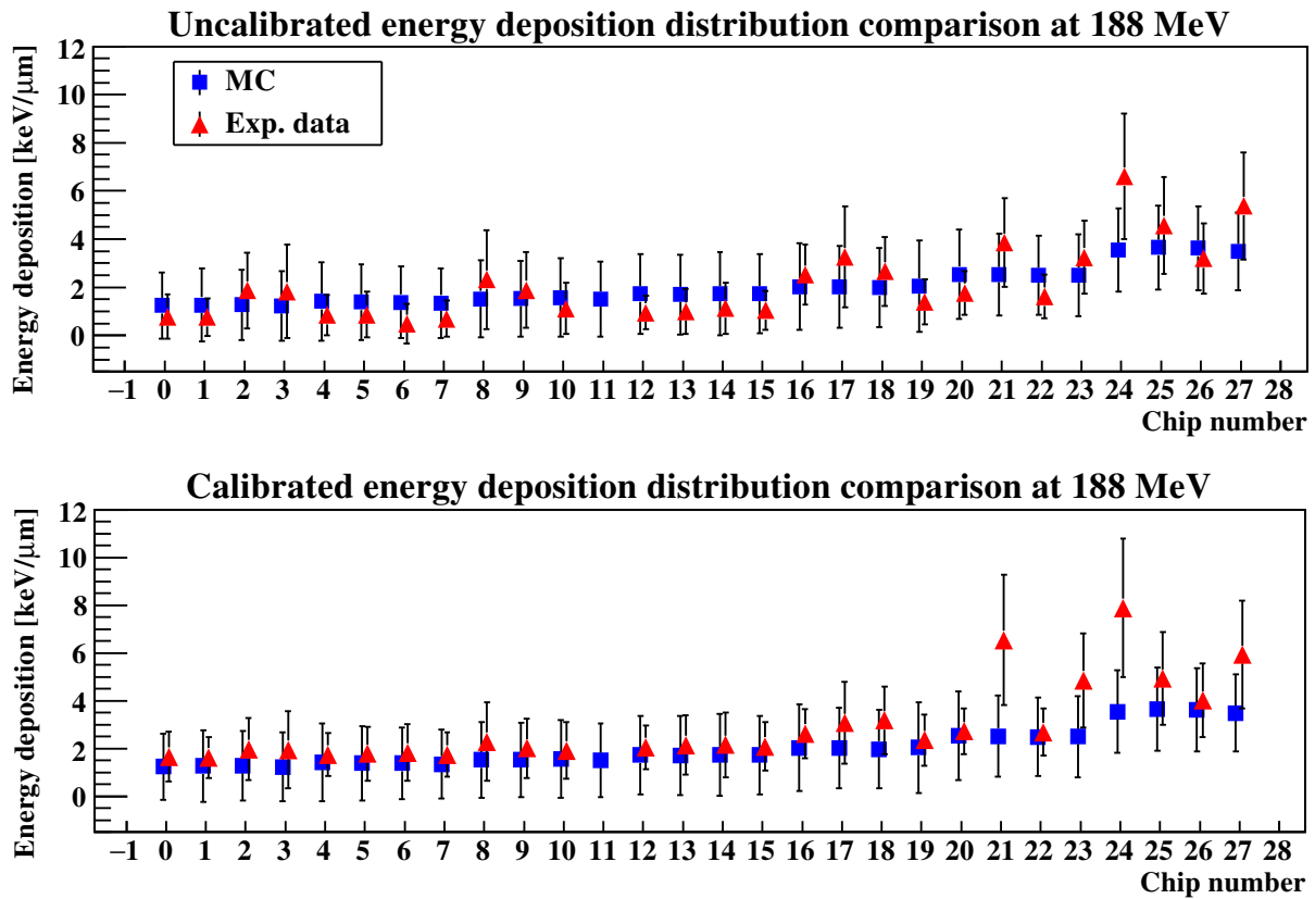
Figure 4.14: Average energy deposition in each chip, applied as validation of the charge diffusion model applied on the MC dataset and for validation of the chip sensitivity calibration on the experimental data. From Pettersen et al. (2017).
