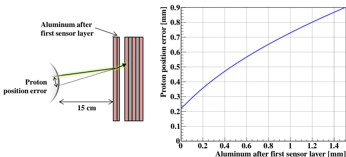
Figure 5.13: Proton position determination error on phantom due to scattering on aluminum carrier board between the first two sensor layers. Left: Schematics of the calculation. Right: Errors from different carrier board thicknesses (and contributions from sensor chips and PCB).
