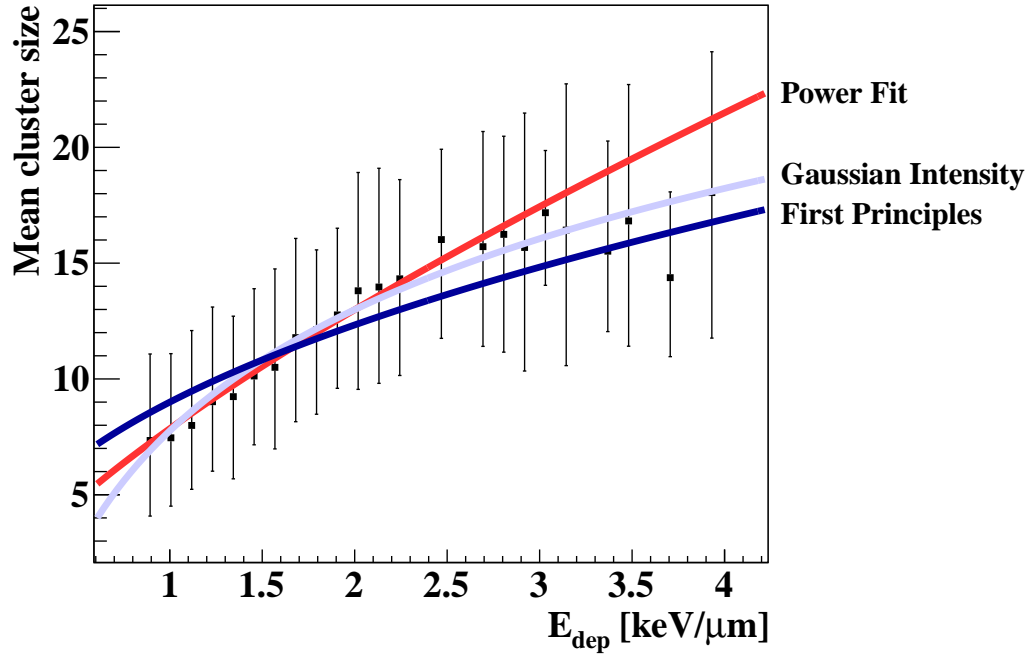
Figure 4.12: Correlation data for E_{dep} and cluster sizes: E_{dep} is calculated using energy-loss tables from Berger et al. (2005). In this graph the mean value and the asymmetric standard deviation values are shown for each of the E_{dep} bins in the histogram of Fig. 4.9, for purposes of curve fitting. Three curves are shown: The analytical charge diffusion model based on first principles, a Gaussian intensity charge distribution model and a power fit to the experimental data using Eq. (4.7).
